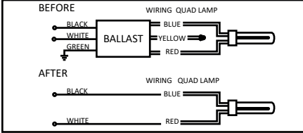
Figure1: Retrofit with One Lamp(G24q Base)
