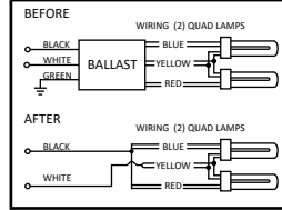
Figure2: Retrofit with Two Lamps(G24q Base)
