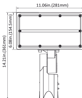
100W(Slipfitter Mount)
